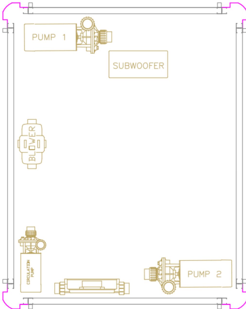
A SIDE PANEL
